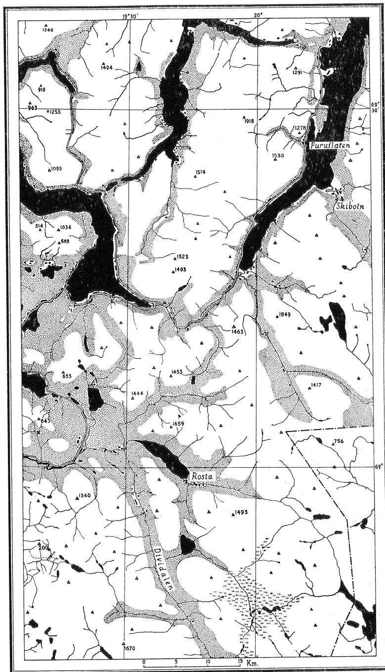
FIG. 1.—General plan of the area in which Drosophilidae were collected. Heights in metres; dotted areas indicate woodlands. (Based on German military map.)
