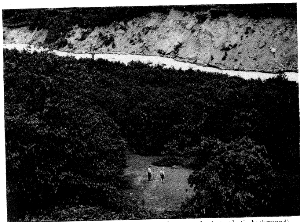
FIG. 2.—Near Furuflaten. Well-grown (30 ft.) alder copse by Lyngselv (in background). D. obscura and Am. alboguttata occurred here. July, 1953.
